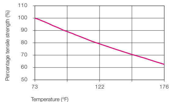
Effect of the temperature on the maximum tensile strength of igubal ® rod end bearings
